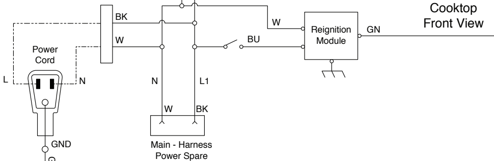
6 Burner Cooktop Schematic
