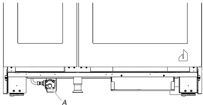
A. Gas pressure regulator
