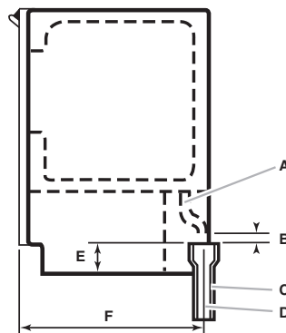
Gravity Drain System Dimensions
