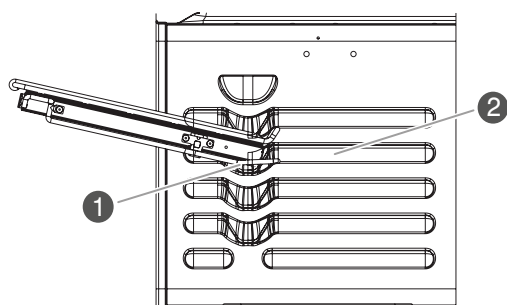
1 "V" cutout 2 Rack guide
