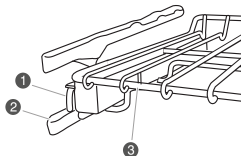
1 Sliding shelf 2 Slide rails 3 Rack
