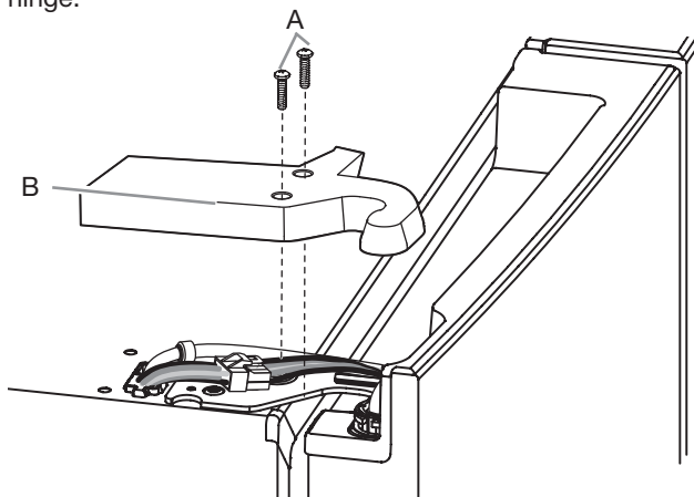
A. Top hinge cover screw
