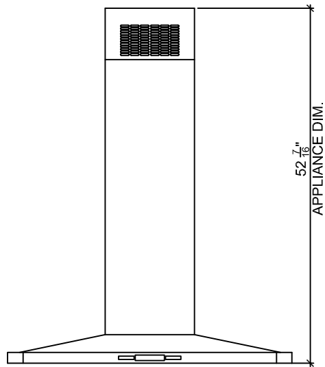
2 FRONT ELEVATION
