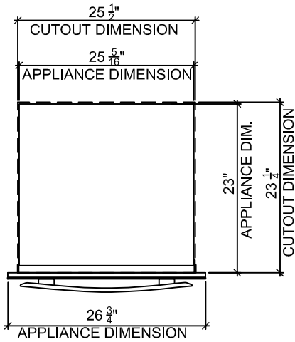
1 PLAN
