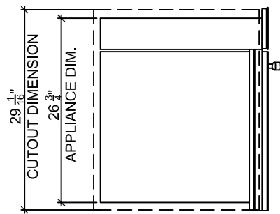
3 SIDE ELEVATION
