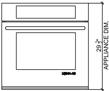
2 FRONT ELEVATION
