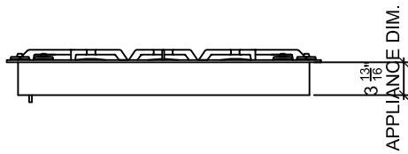
2 FRONT ELEVATION
