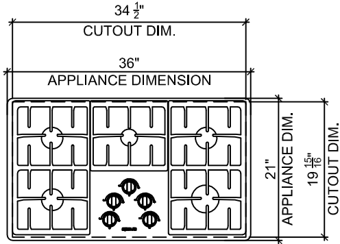
1 PLAN
