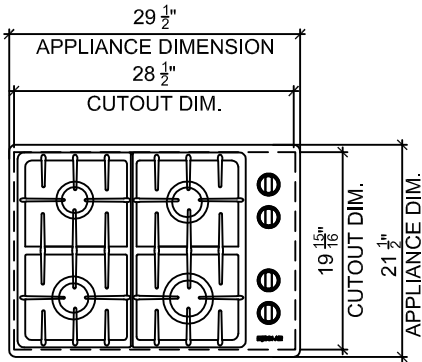
1 PLAN
