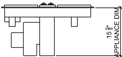
2 FRONT ELEVATION
